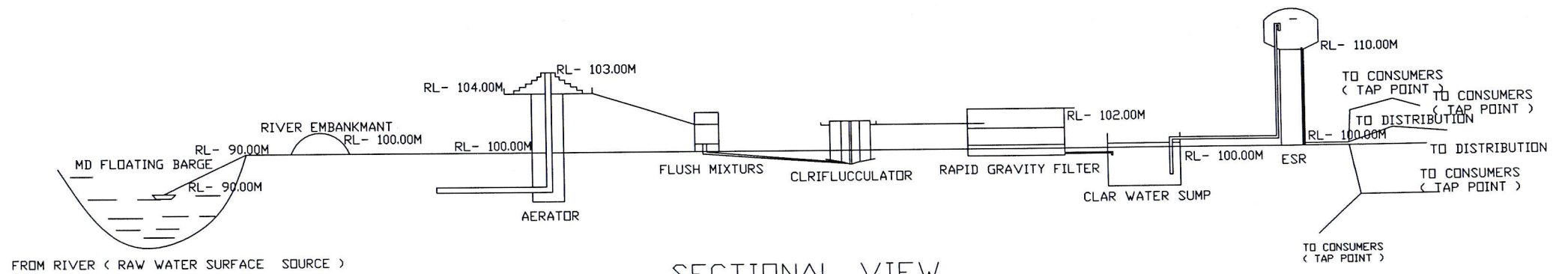
SECTIONAL VIEW
